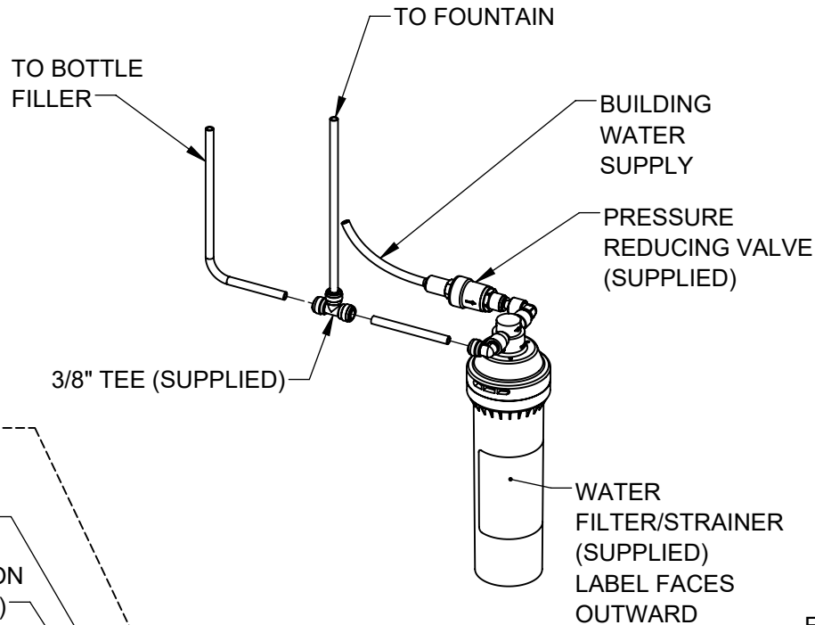
WATERWAY DIAGRAM
